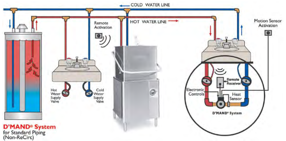
Figure 8. Demand circulation diagram. Photo Credit: Taco (Modified)
