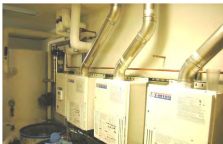
Figure 28. Tankless heaters, controller and 200 gallon storage tank.
