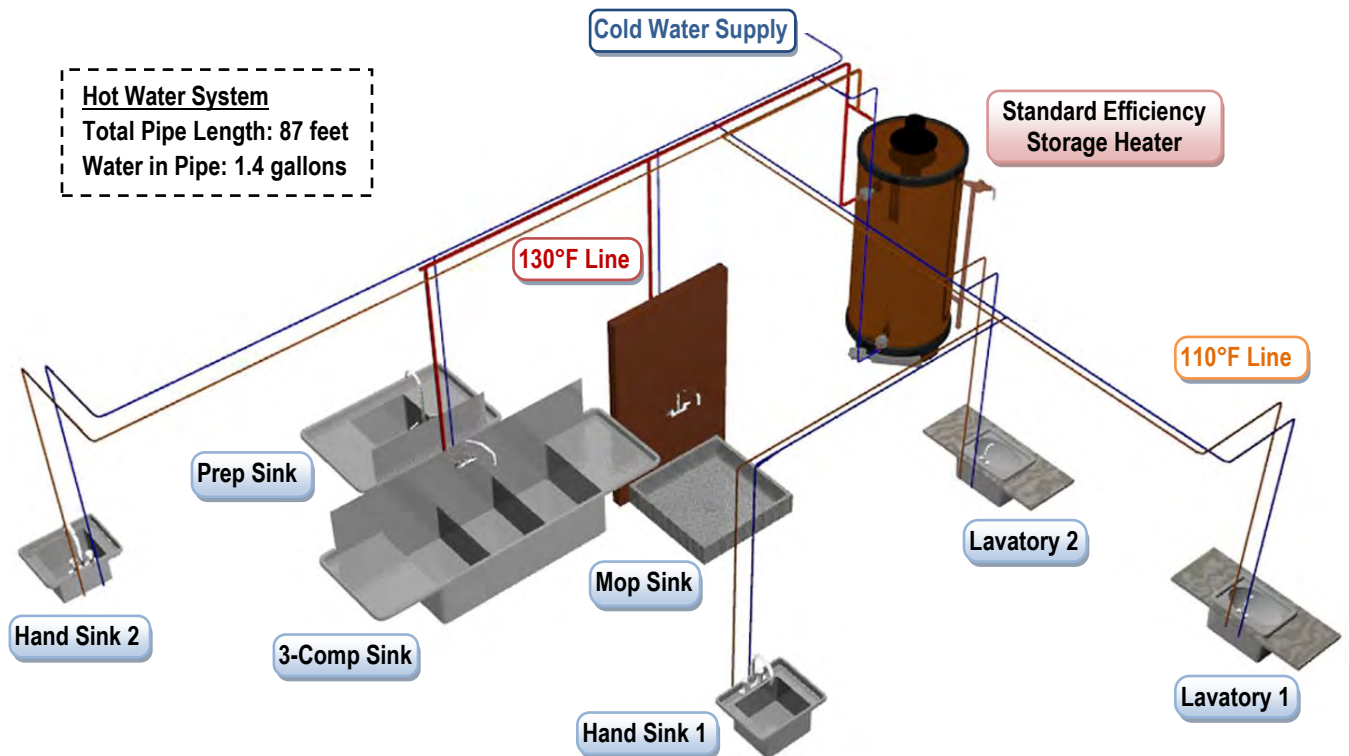
Figure 42. Configuration A: Hot-water-system design of a conventional quick-service restaurant.
